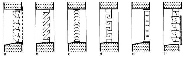
② Ventilation openings: a = self opening; b,c,d,e = non-moving; d = for dark rooms; f = manually operated
